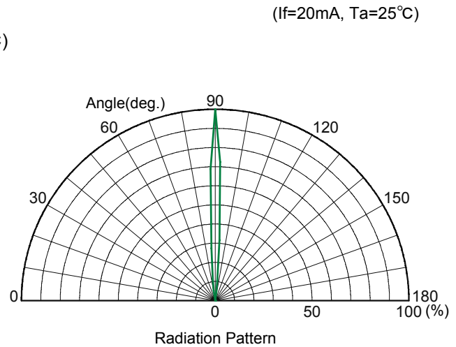
Radiation Pattern
