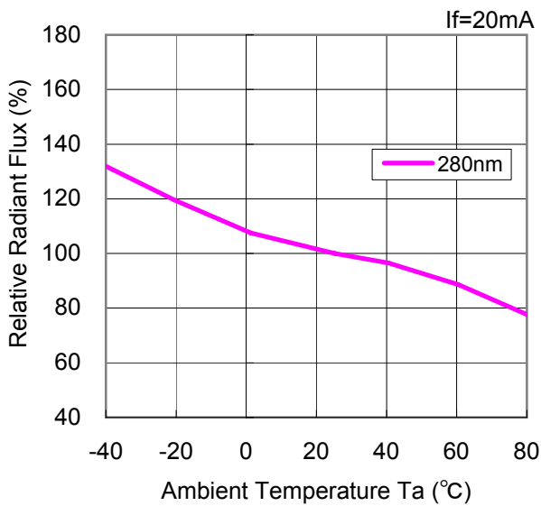
Radiant Flux vs Ambient Temperature
