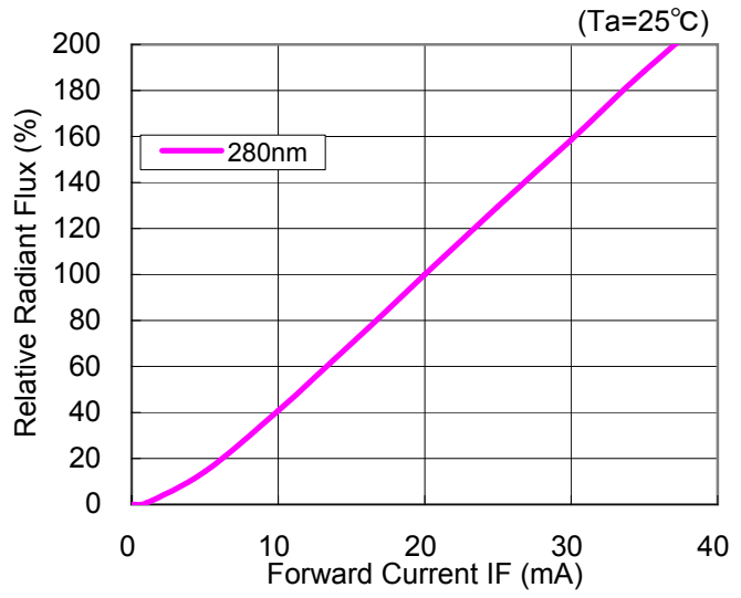
Forward Current vs Radiant Flux
