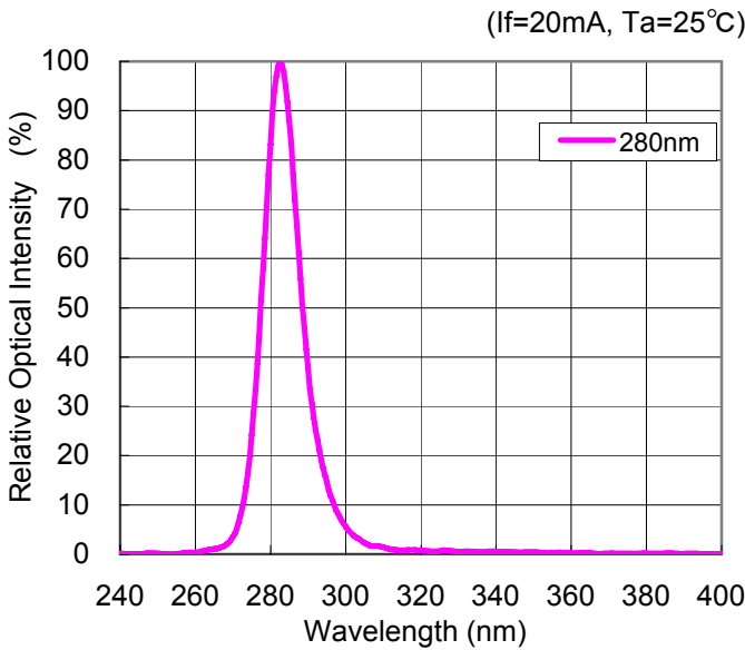
Relative Intensity vs Peak Wavelength
