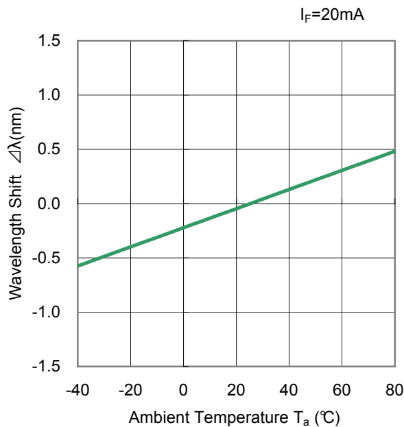
Wavelength Shift vs Ambient Temperature
