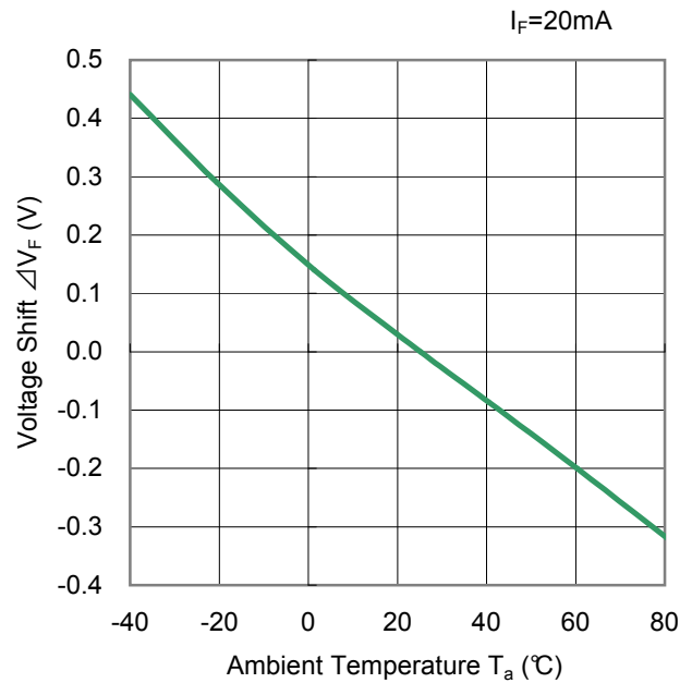
Voltage Shift vs Ambient Temperature
