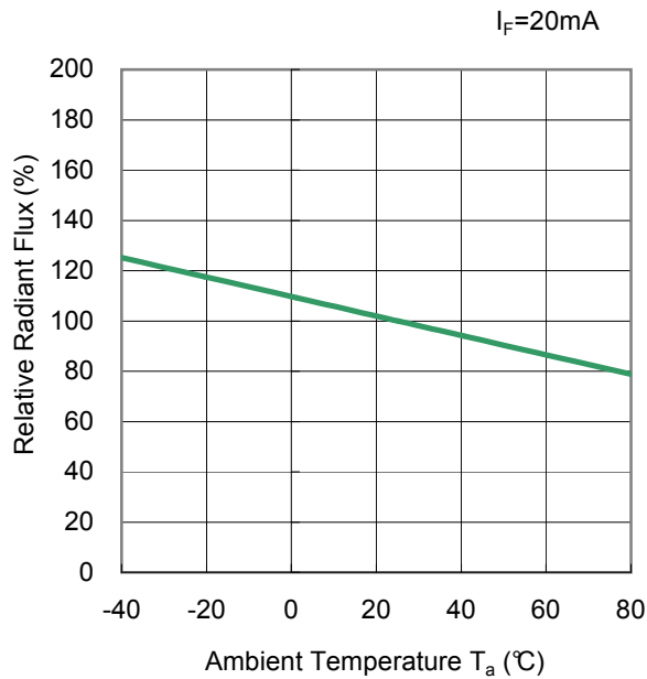
Radiant Flux vs Ambient Temperature
