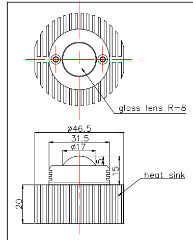
Outer Dimension (Unit:mm)
