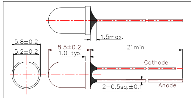
Outer Dimension (Unit:mm)
