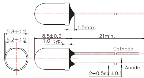
Figure 2: \Phi 5 Mold type 02
