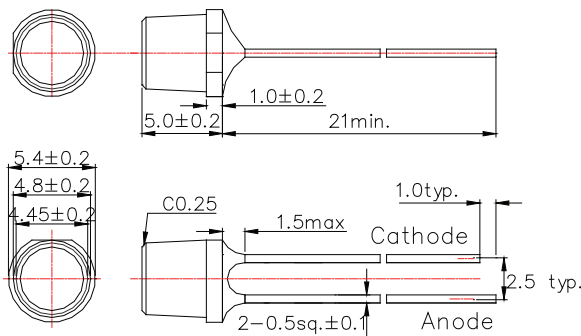
Figure 5: \Phi 5 Mold type 05
