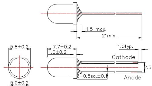
Figure 4: \Phi 5 Mold type 04
