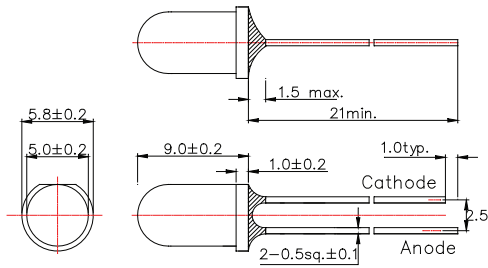
Figure 1: \Phi 5 Mold type 01
