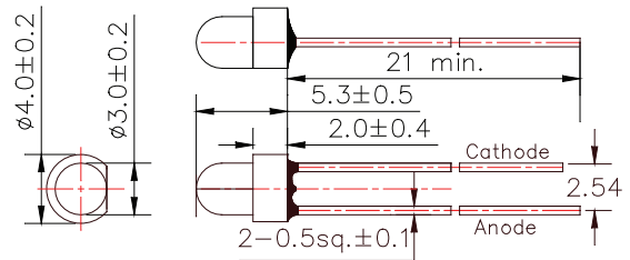
Figure 11: \Phi 5 Mold type 36
