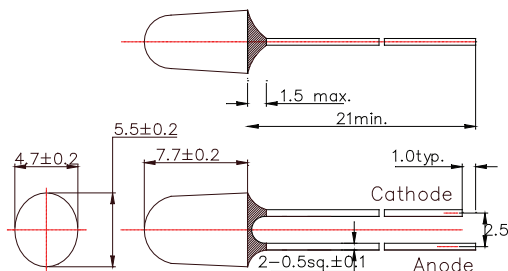
Figure 7: \Phi 5 Mold type 09
