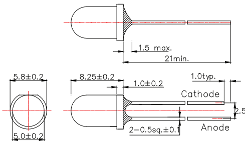
Figure 3: \Phi 5 Mold type 03
