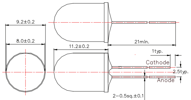
Figure 13: \Phi 5 Mold type 82
