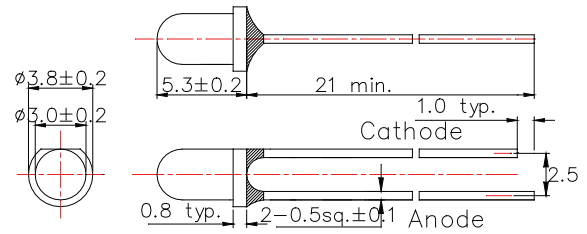
Figure 9: \Phi 5 Mold type 33
