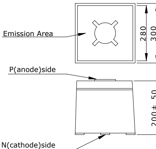
Fig.2 Chip size and Emission Area
