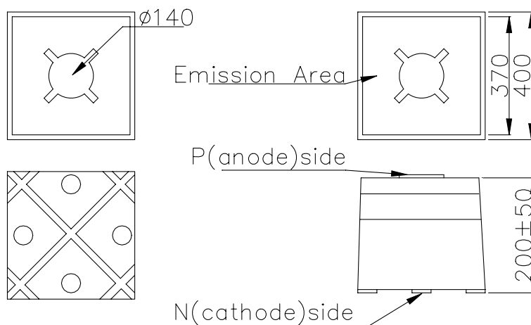
Fig.1 Electrode Pattern
