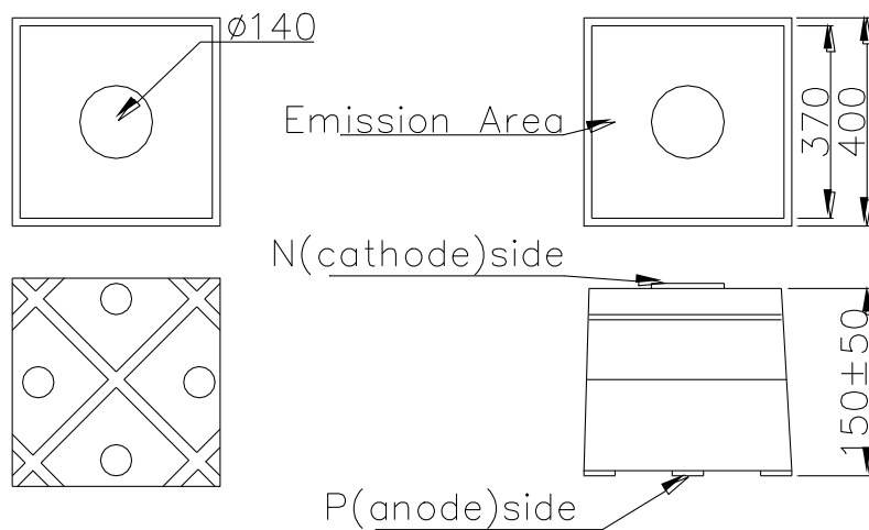
Fig.1 Electrode Pattern
