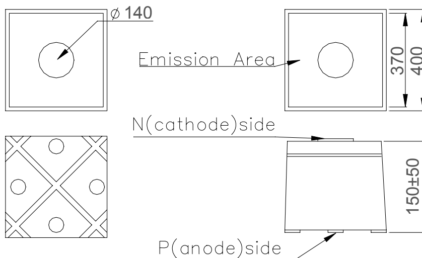
Fig.1 Electrode Pattern
