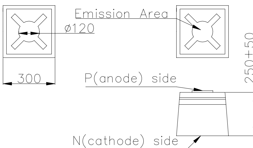
Fig.1 Electrode Pattern
