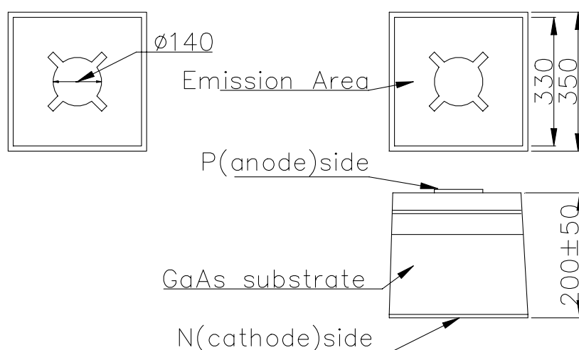
Fig.1 Electrode Pattern
