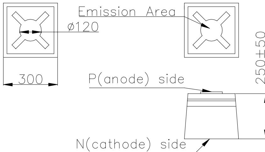
Fig.1 Electrode Pattern
