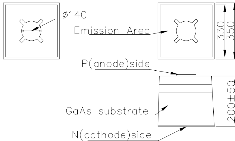
Fig.1 Electrode Pattern
