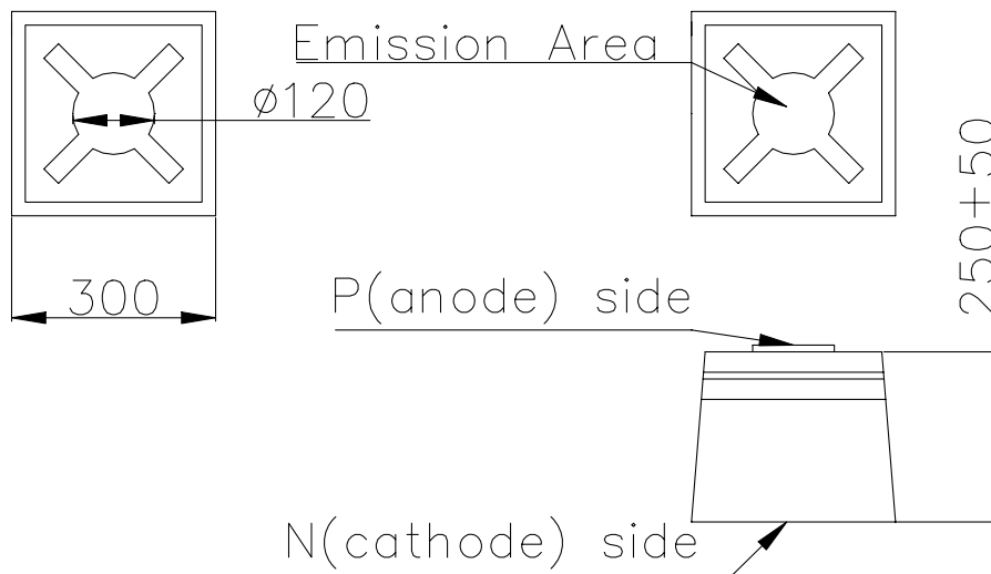
Fig.1 Electrode Pattern
