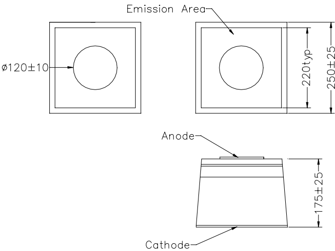
Fig.1 Electrode Pattern
