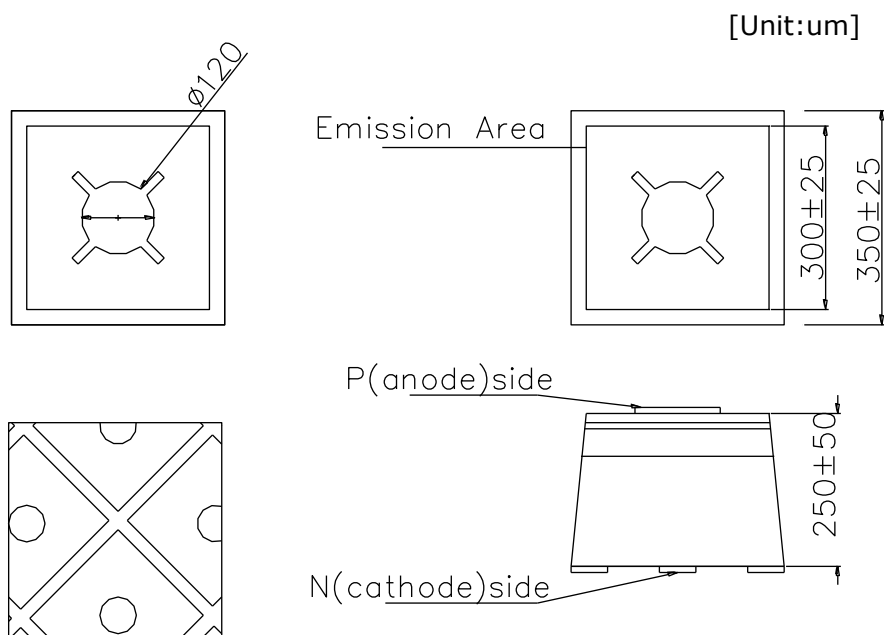
Fig.1 Electrode Pattern
