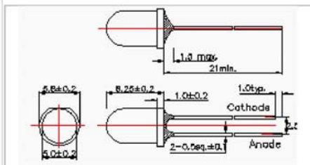
Figure 5 Ö5 Mold type 05
