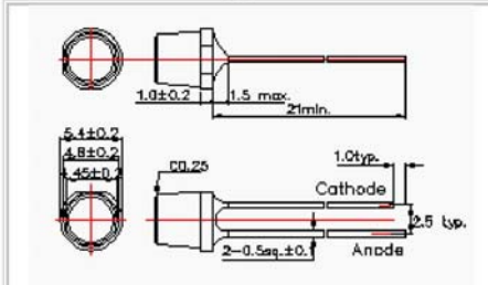
Figure 7 Ö5 Mold type 09
