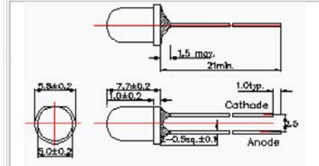
Figure 6 Ö5 Mold type 06
