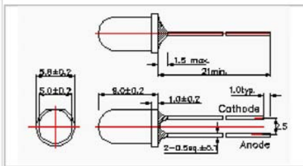
Figure 3 Ö5 Mold type 03
