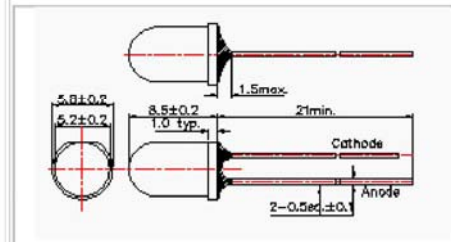
Figure 4 Ö5 Mold type 04
