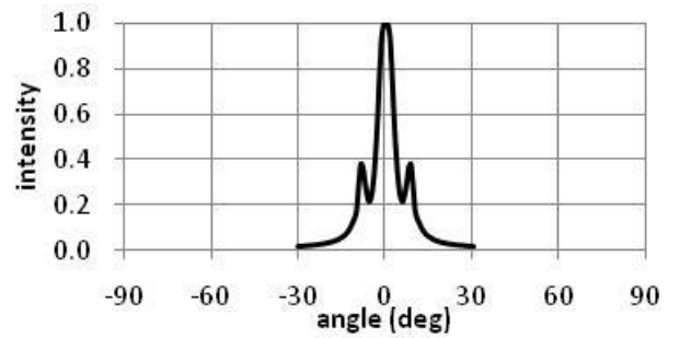
Figure-8 \Phi 5 Mold (Type46)
