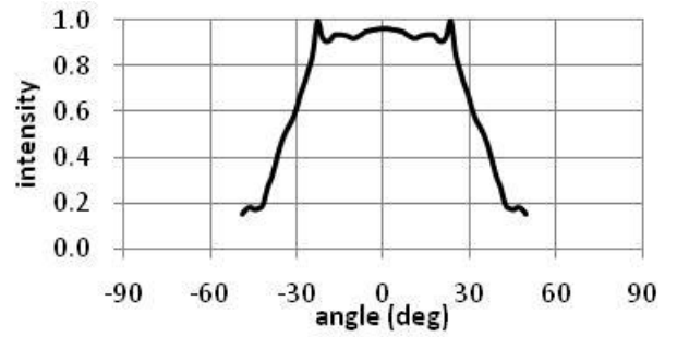
Figure-6 \Phi 5 Mold (Type06)
