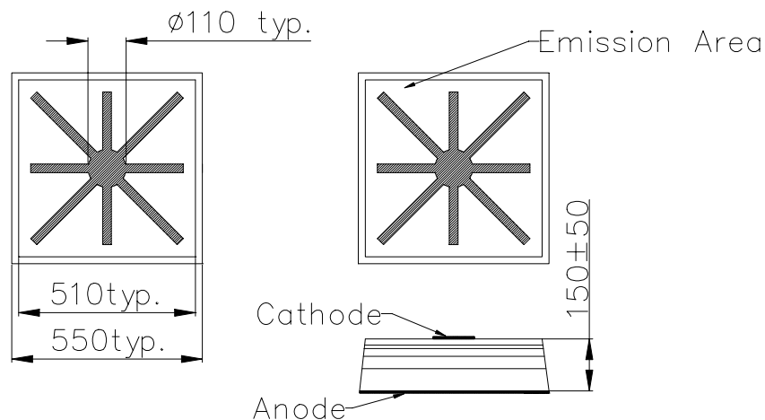
Fig.1 Electrode Pattern
