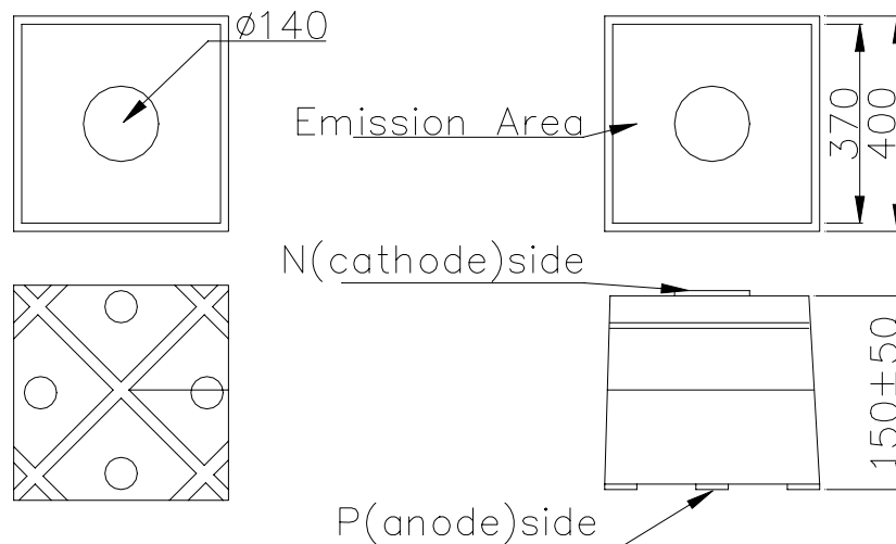
Fig.1 Electrode Pattern
