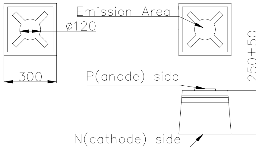
Fig.1 Electrode Pattern
